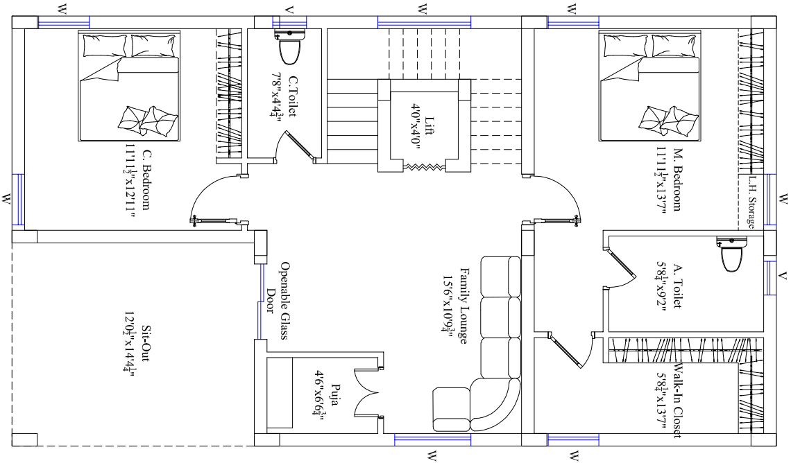
F.F. Plan Slab Area : 1153.875 Sq.Ft.
