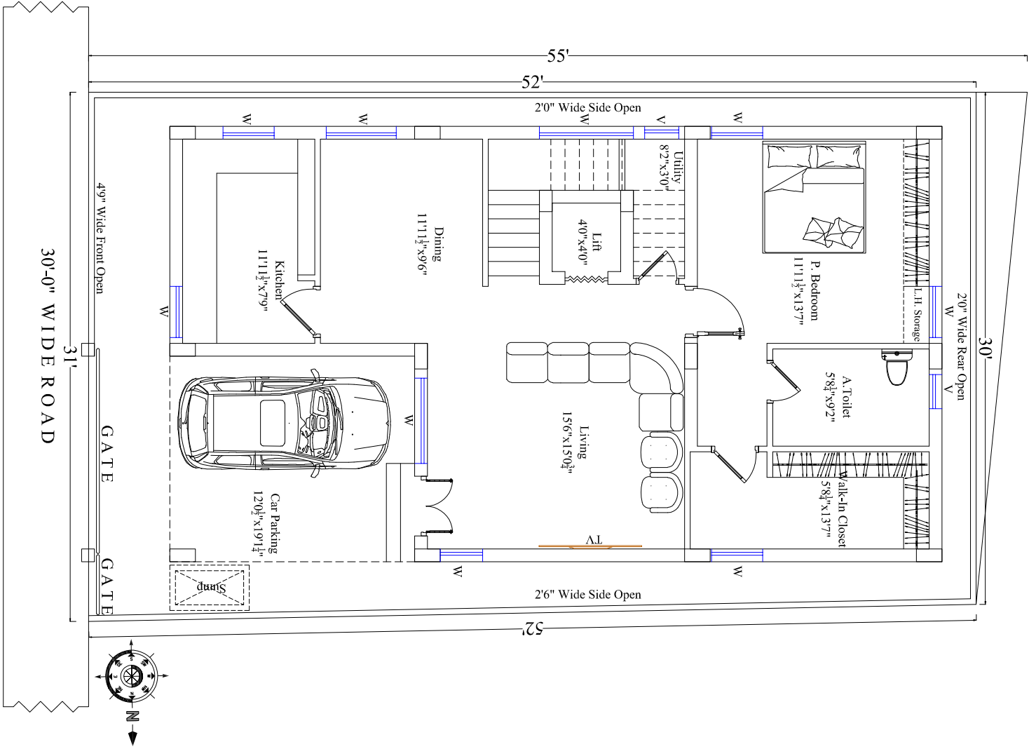
G.F. Plan Slab Area : 1153.875 Sq.Ft.
